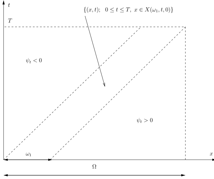
Figure 5.6: Sign of the time derivative of \psi .
