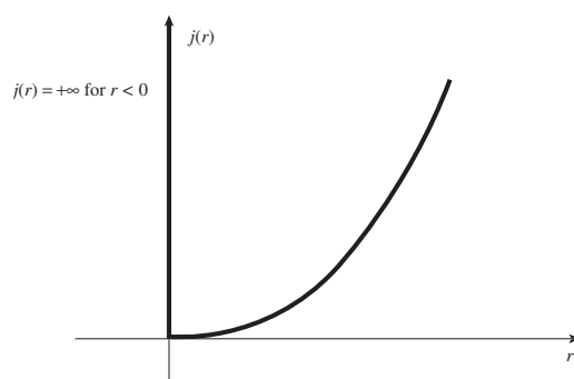
Figure 1 The function j .
